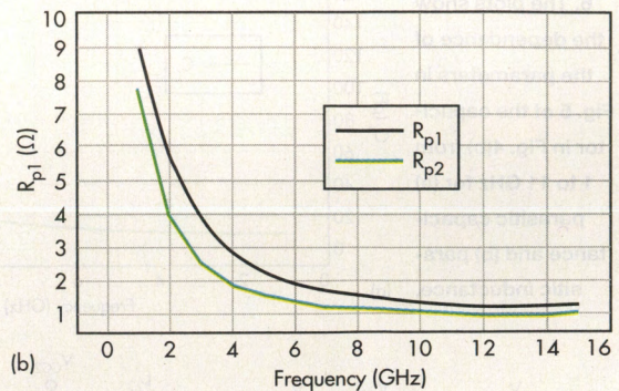
3. These curves show the dependence of the circuit parameters of Fig. 2(b) for (a) the effective inductance, L_s , and (b) resistances added by the parasitic capacitances.
