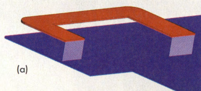
1. These images portray (a) the output impedance-matching inductor and (b) the power bias inductor on the laminate of the PAM.
