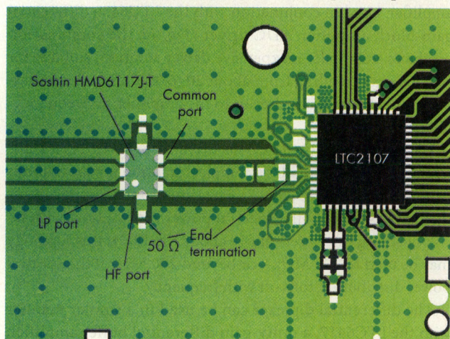
3. The artwork here represents circuitry that can be fabricated for the HMD6117J-T/LTC2107 combination devices.
