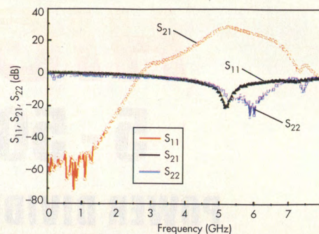
12. The plots show measured S_{11} , S_{21} , and S_{22} for the PAM.
