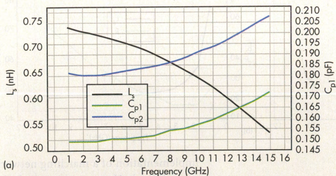
3. These curves show the dependence of the circuit parameters of Fig. 2(b) for (a) the effective inductance, L_s , and (b) resistances added by the parasitic capacitances.
