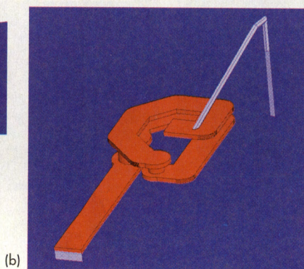
1. These images portray (a) the output impedance-matching inductor and (b) the power bias inductor on the laminate of the PAM.
