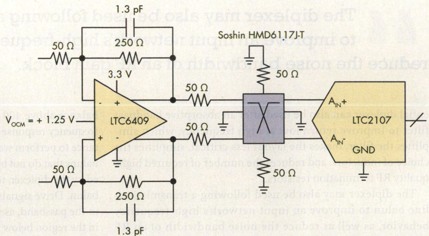
2. This source-terminated, dc-coupled driver can be used to 100 MHz.
