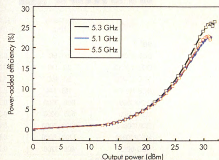
14. These plots reveal the measured dependence of PAE on the PAM's output power at 5.1, 5.5, and 5.7 GHz.
