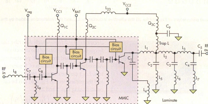
7. This is a schematic circuit diagram representing the three-stage PA on the MMIC.
