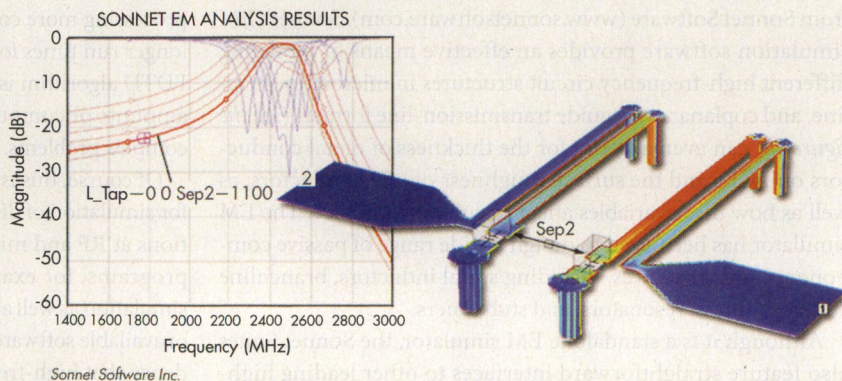
The free-of-charge SonnetLite EM simulation software was used to design this edge-coupled microstrip bandpass filter. (Courtesy of Sonnet Software)
